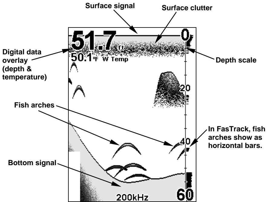
Sonar Page showing full sonar chart mode.
